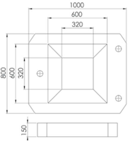
DALLE SIMPLE ABSORPTION
