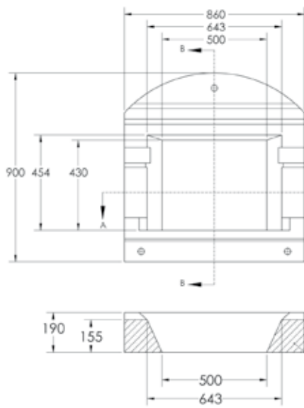
DALLE DOUBLE ABSORPTION
